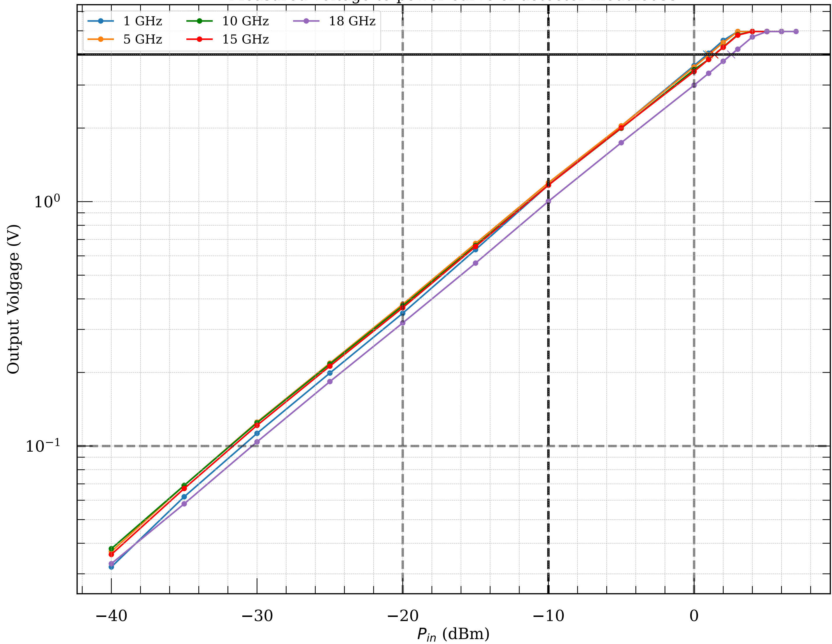
Measured voltage-to-power curve of detector module059
